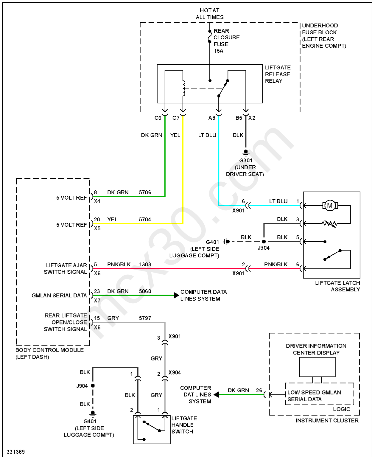
Fig. 79: Liftgate Release Circuit
