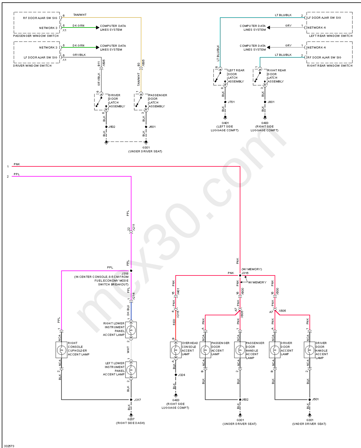
Fig. 41: Courtesy Lamps Circuit (2 of 2)
