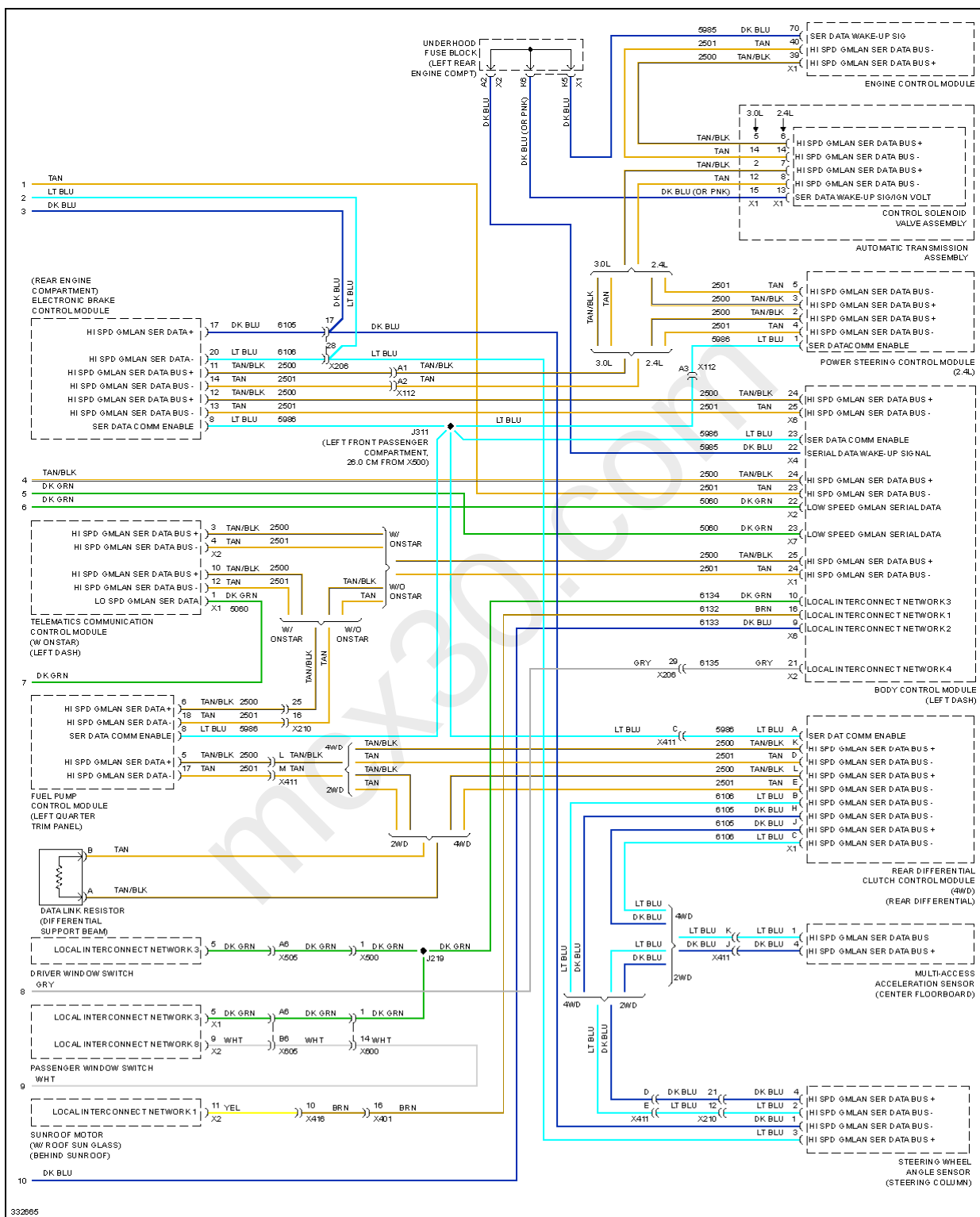
Fig. 13: Computer Data Lines Circuit (2 of 2)
