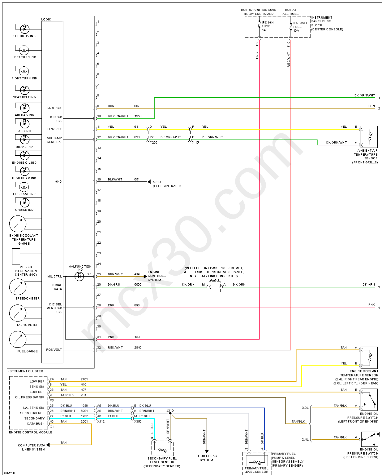
Fig. 38: Instrument Cluster Circuit (1 of 2)
