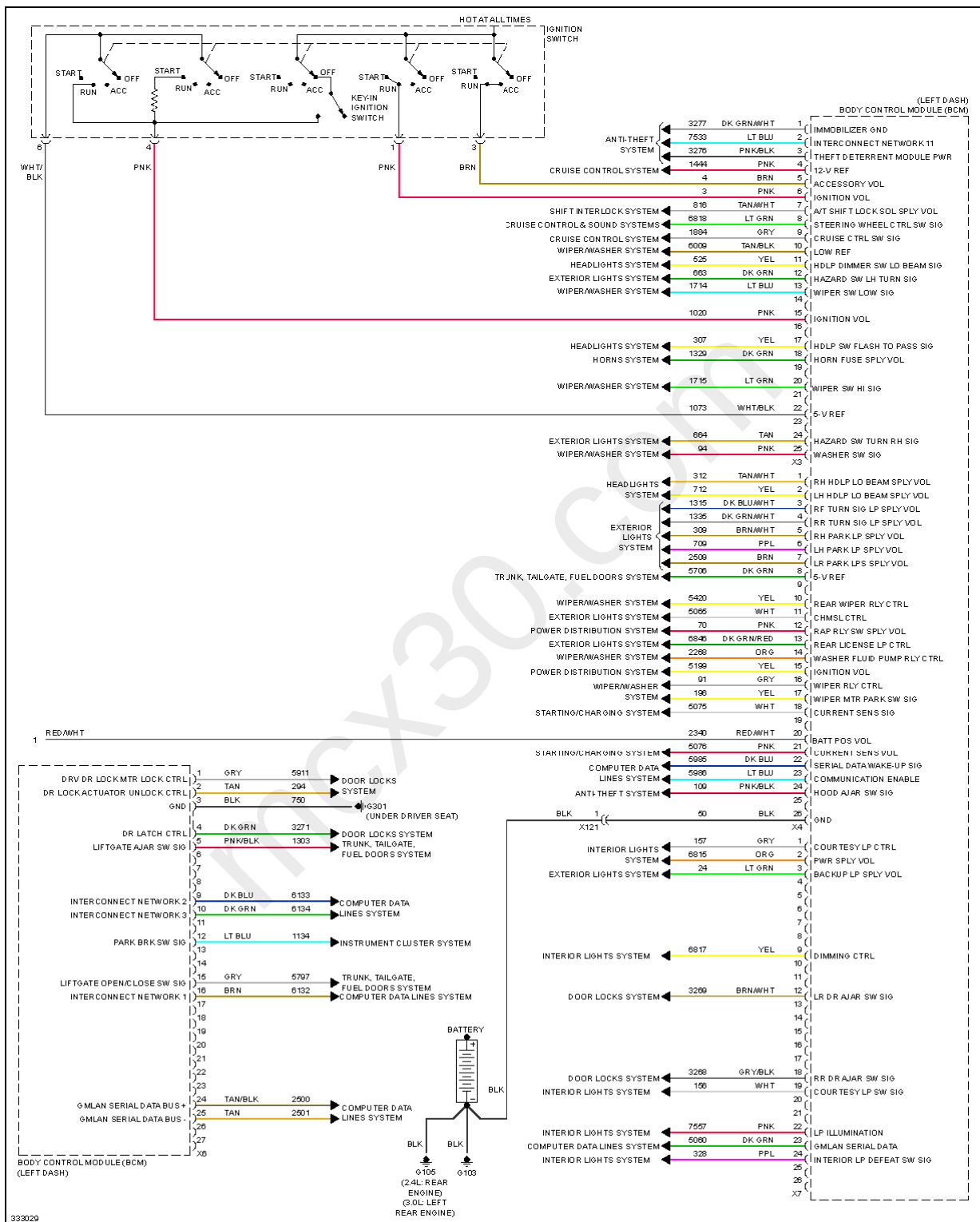
Fig. 11: Body Control Modules Circuit (2 of 2)
