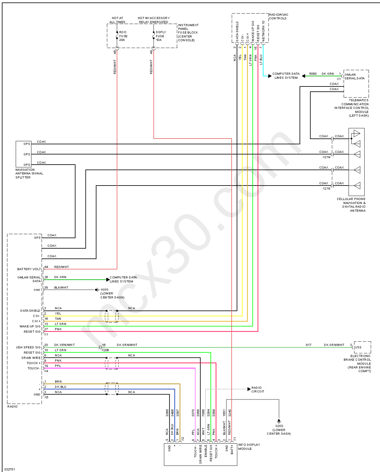
Fig. 46: Navigation Circuit
