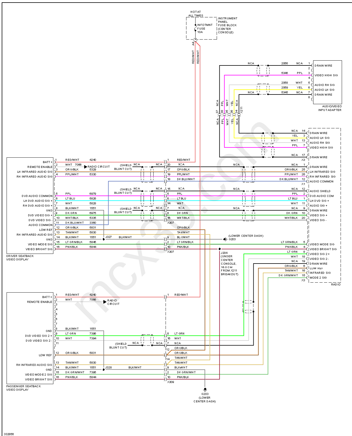
Fig. 68: Video System Circuit
