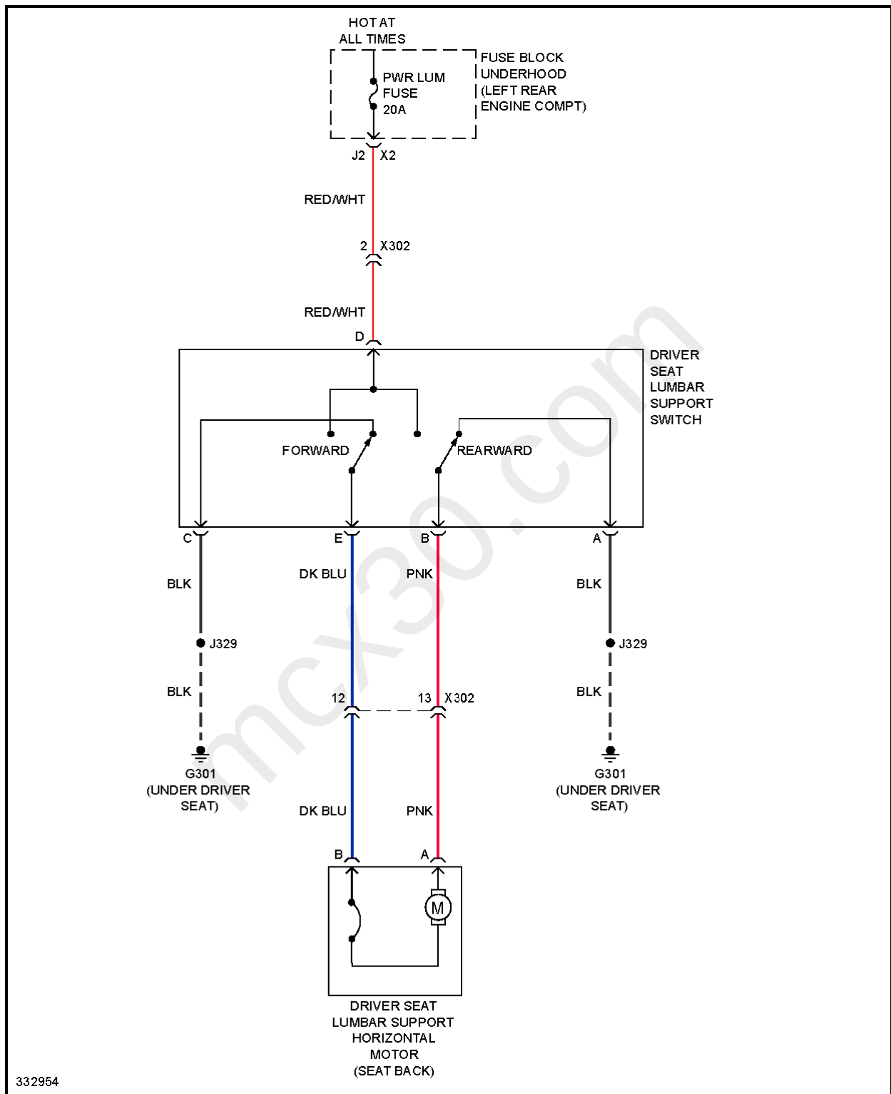
Fig. 58: Driver's Lumbar Circuit
