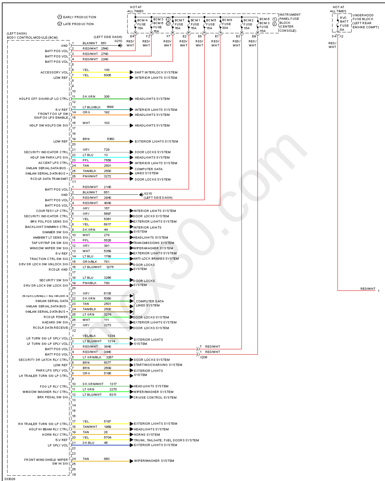
Fig. 10: Body Control Modules Circuit (1 of 2)
