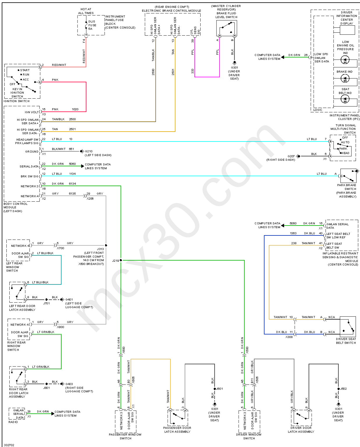
Fig. 81: Warning Systems Circuit
