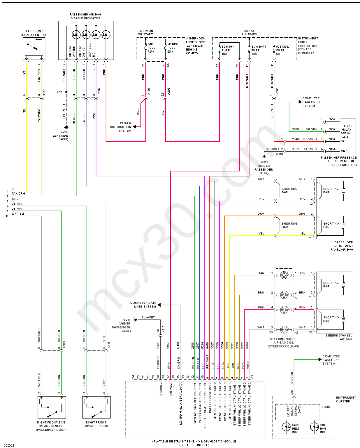
Fig. 74: Supplemental Restraints Circuit (2 of 2)
