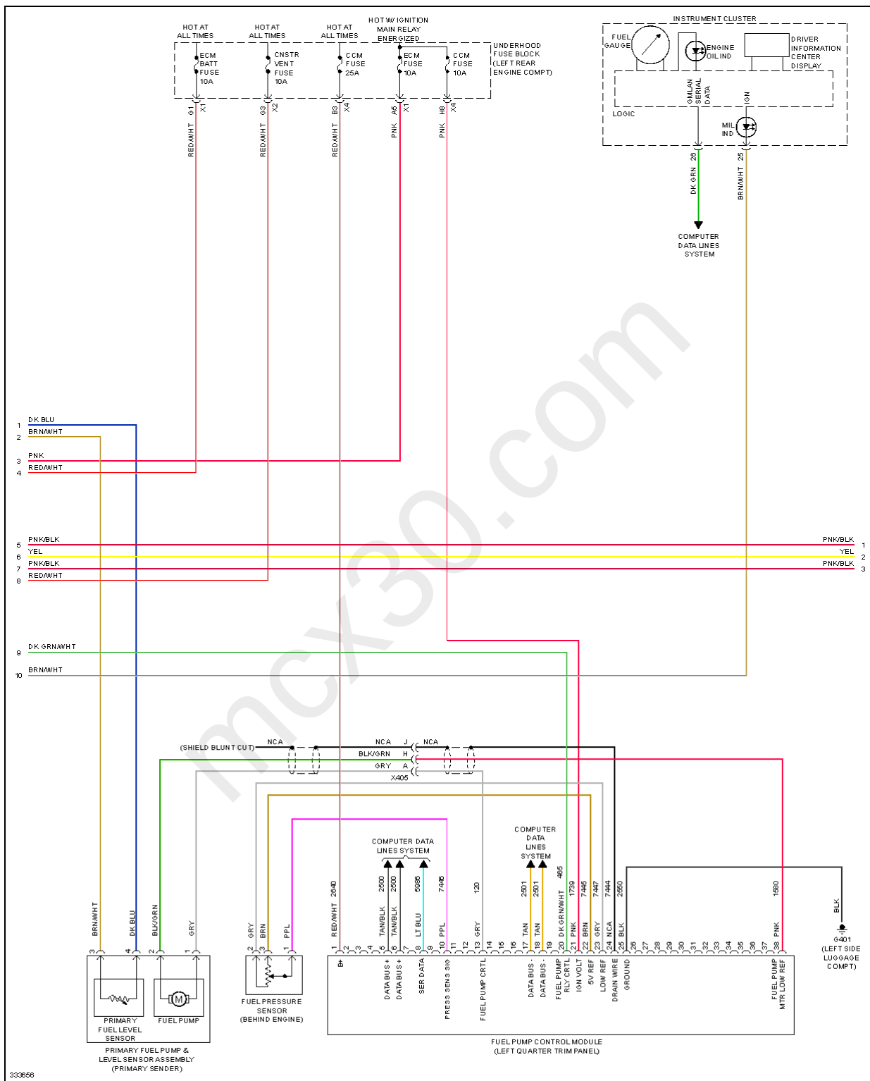
Fig. 20: 2.4L VIN W, Engine Performance Circuit (2 of 5)
