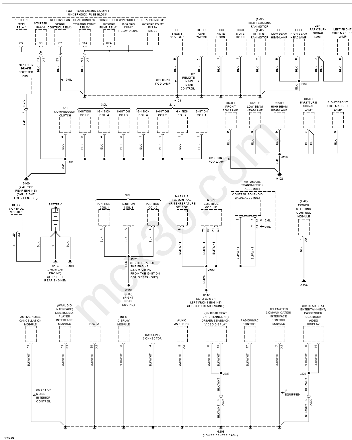
Fig. 32: Ground Distribution Circuit (1 of 4)
