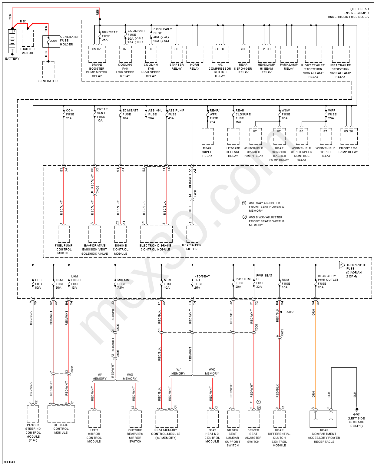
Fig. 49: Power Distribution Circuit (1 of 4)
