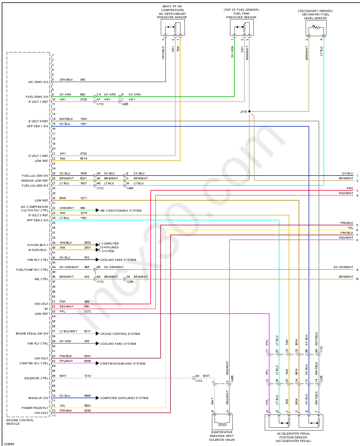
Fig. 19: 2.4L VIN W, Engine Performance Circuit (1 of 5)
