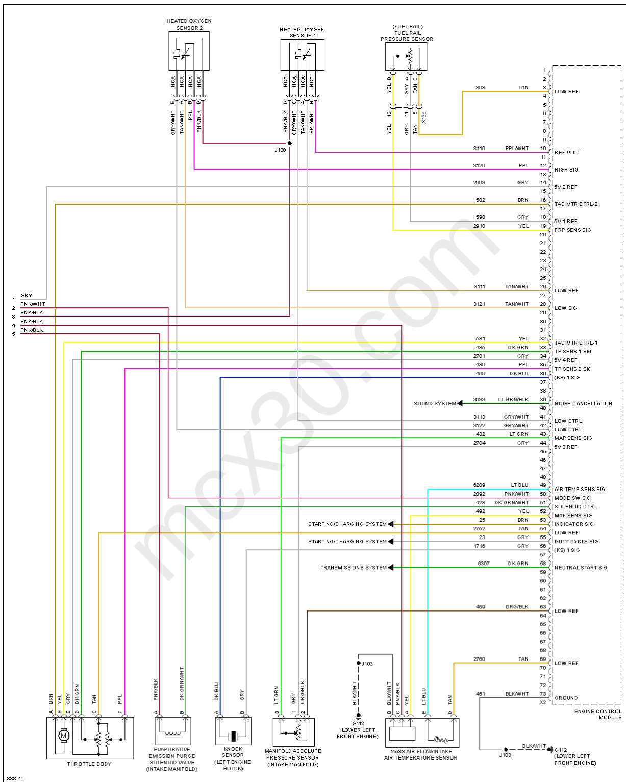
Fig. 23: 2.4L VIN W, Engine Performance Circuit (5 of 5)
