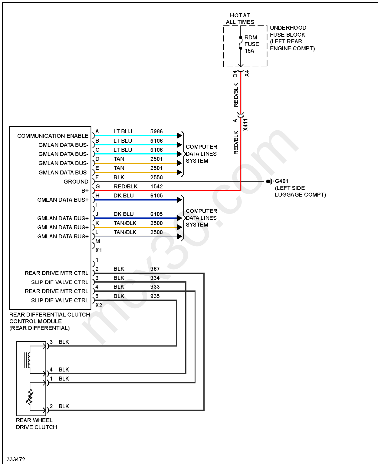
Fig. 76: 2.4L VIN W, Rear Differential Lock Circuit
