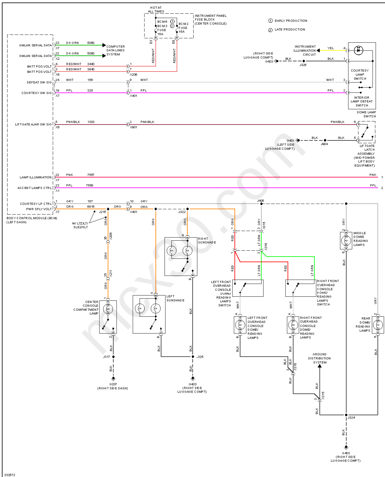
Fig. 40: Courtesy Lamps Circuit (1 of 2)
