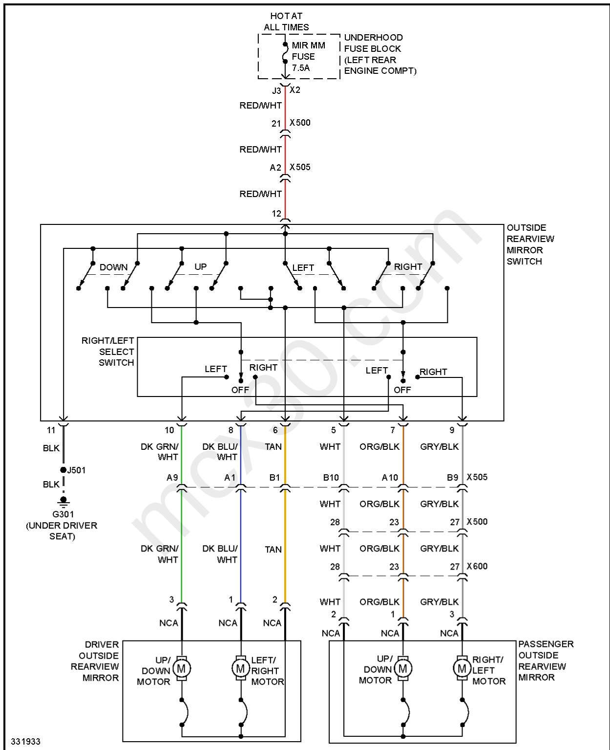
Fig. 57: Power Mirrors Circuit
