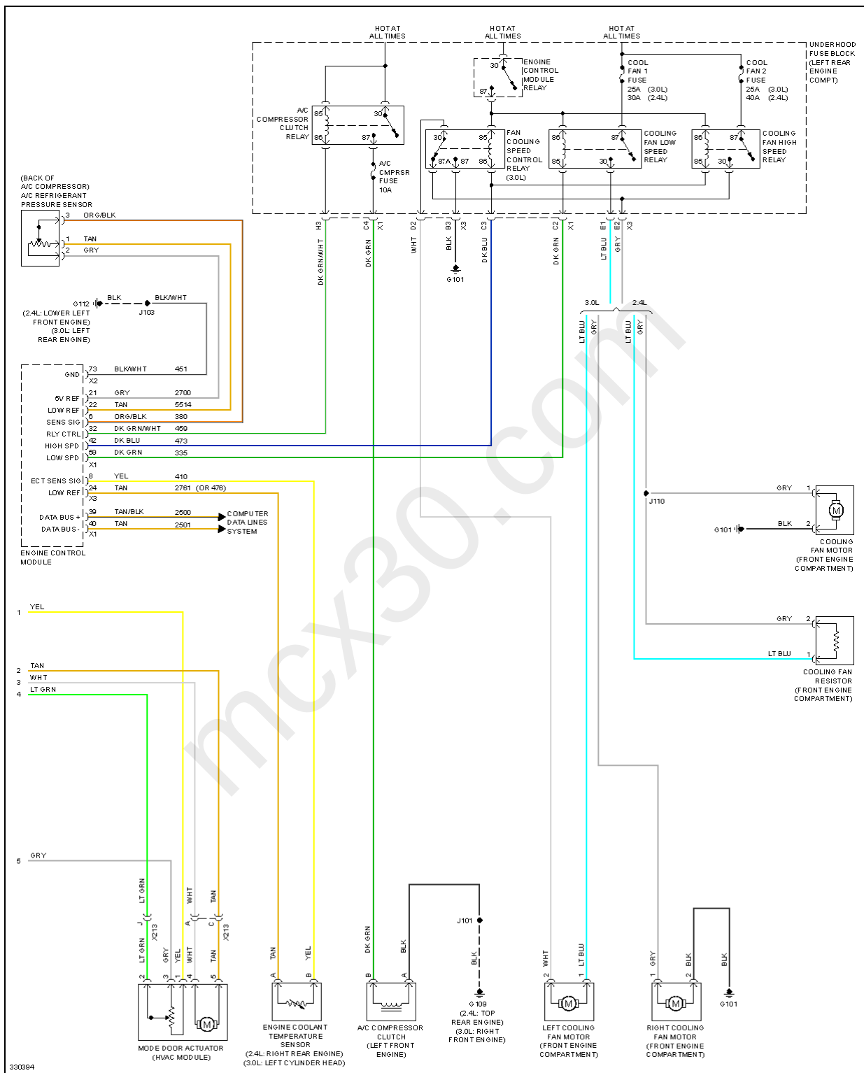
Fig. 5: Manual A/C Circuit (2 of 2)
