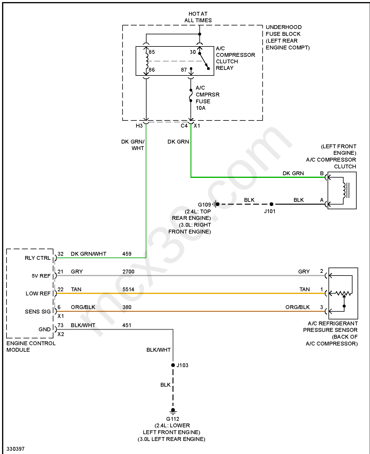
Fig. 3: Compressor Circuit
