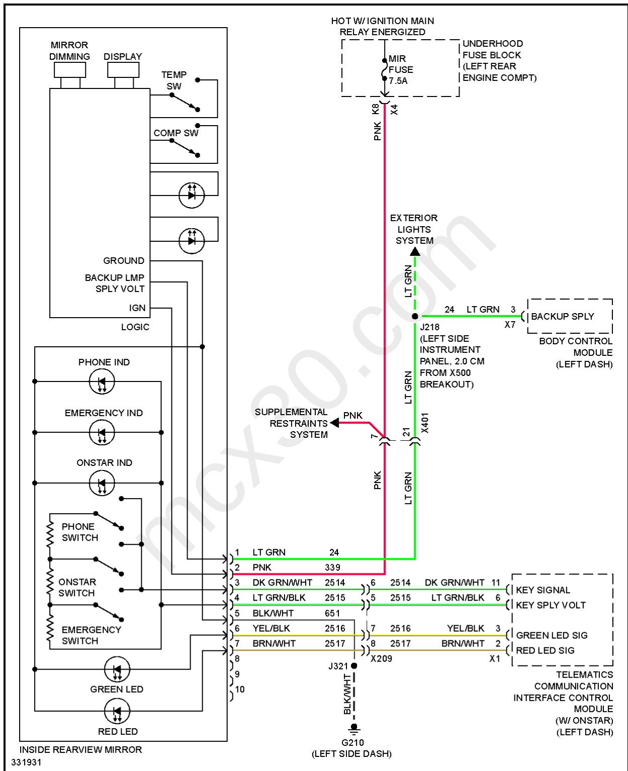
Fig. 56: Electrochromic Mirror Circuit, W/O Rear View Camera
