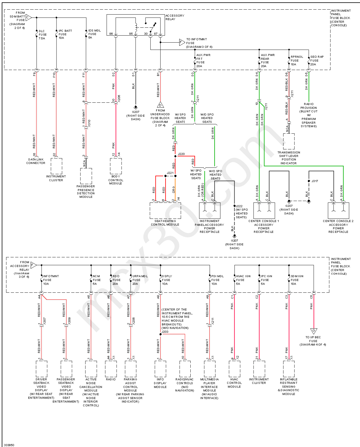
Fig. 51: Power Distribution Circuit (3 of 4)
