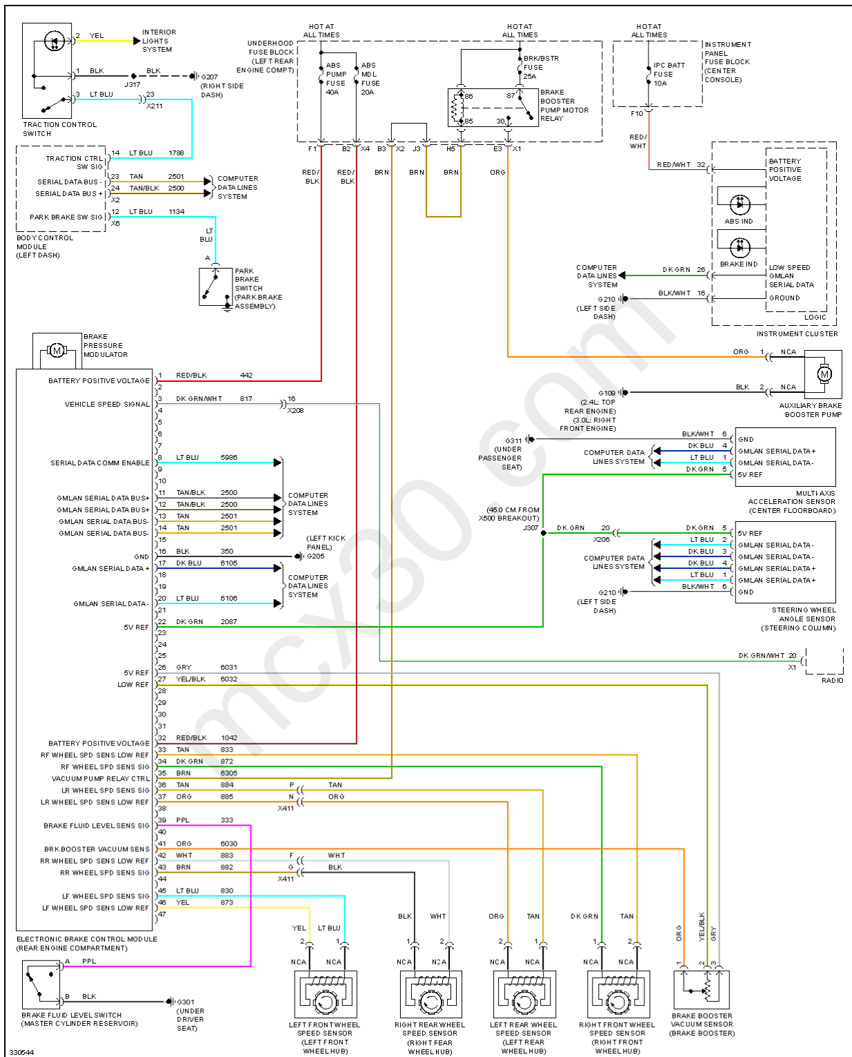
Fig. 6: Anti-lock Brakes Circuit
