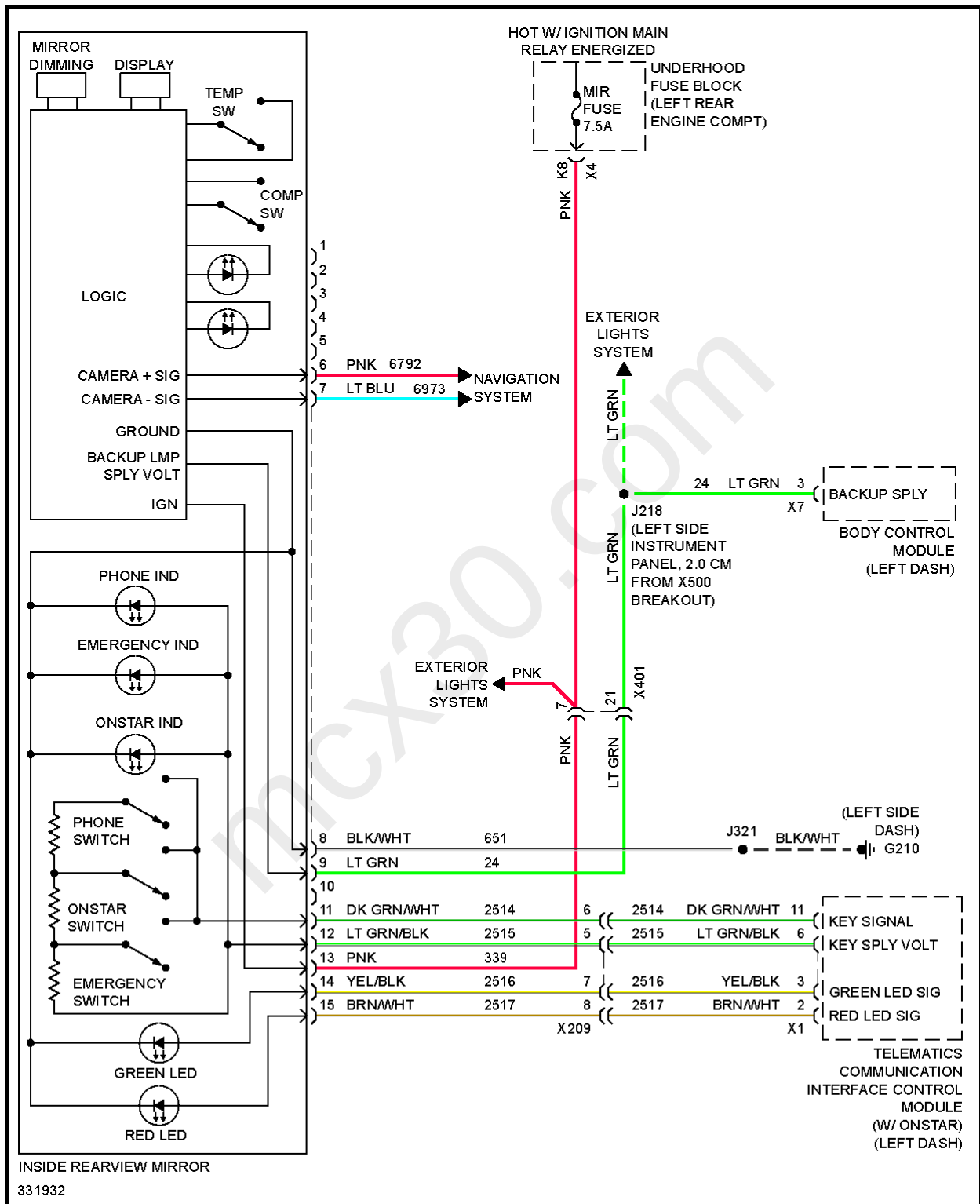
Fig. 55: Electrochromic Mirror Circuit, W/ Rear View Camera
