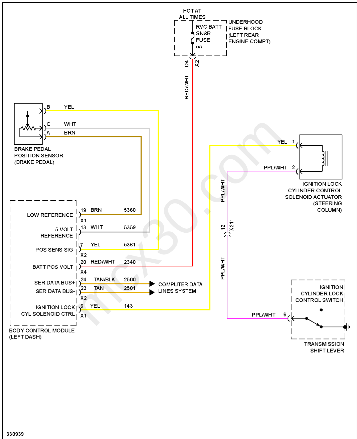
Fig. 69: Ignition Lock Solenoid Circuit
