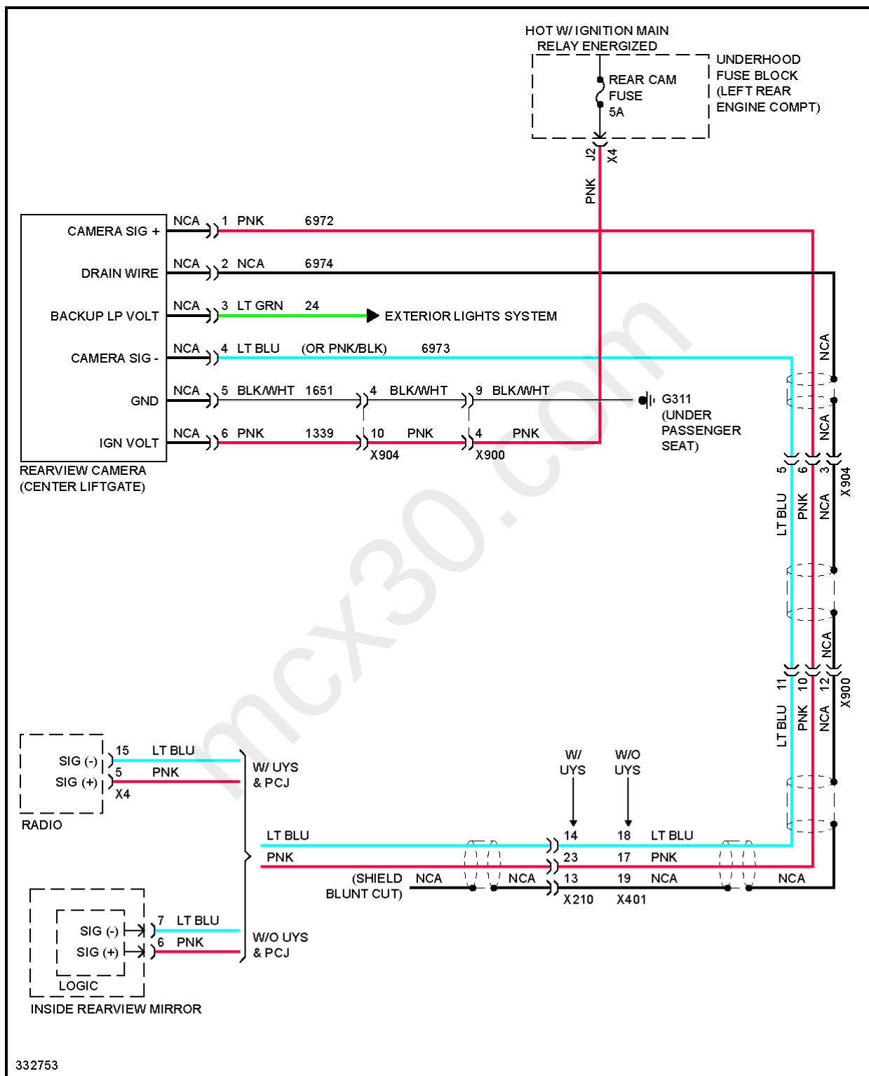
Fig. 48: Rear View Camera Circuit
