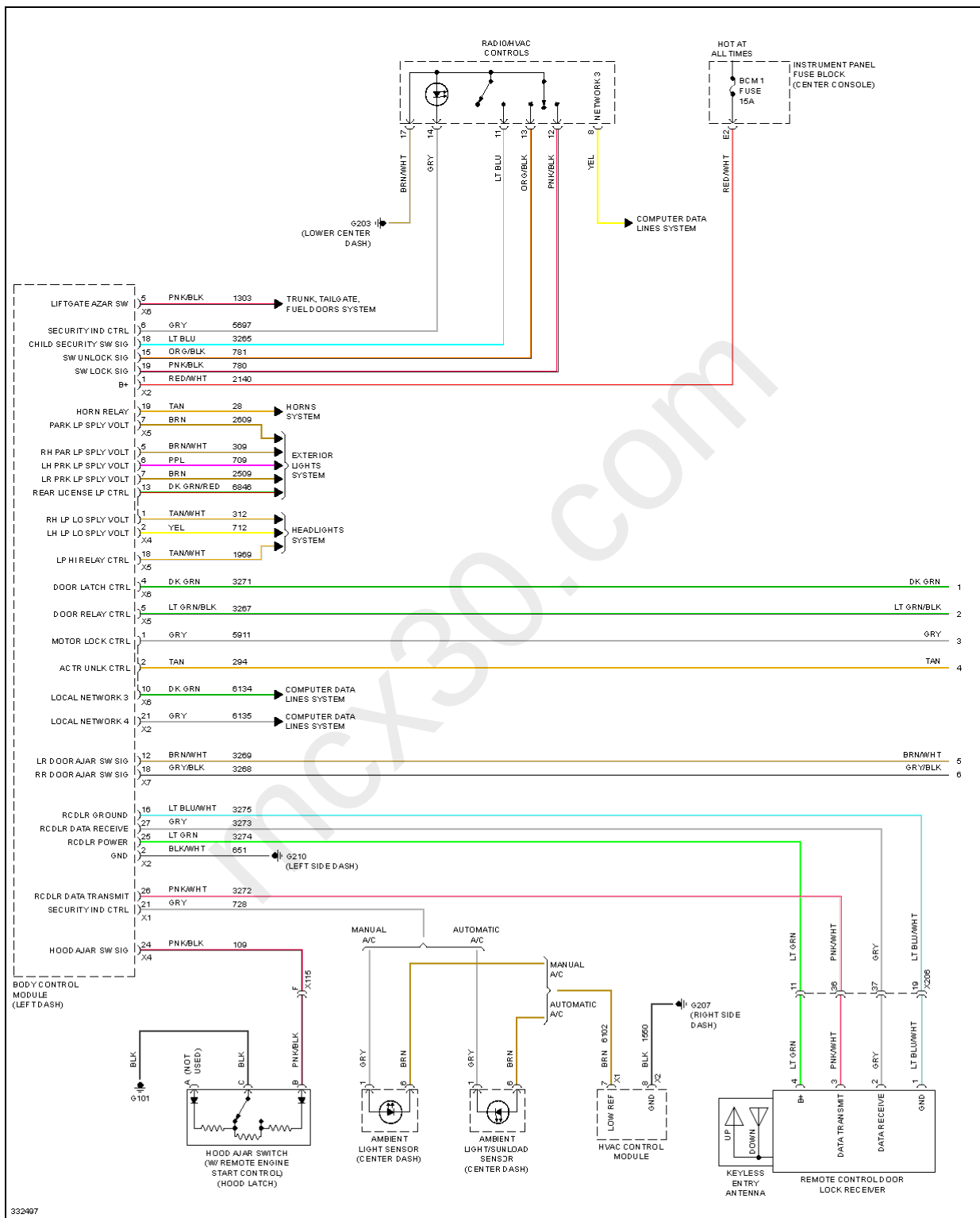
Fig. 53: Power Door Locks Circuit (1 of 2)
