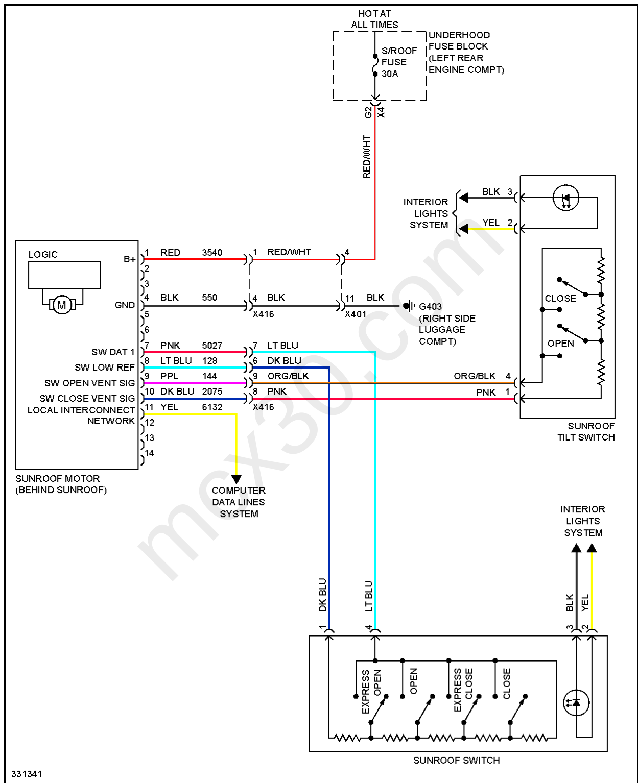
Fig. 63: Power Top/Sunroof Circuit
