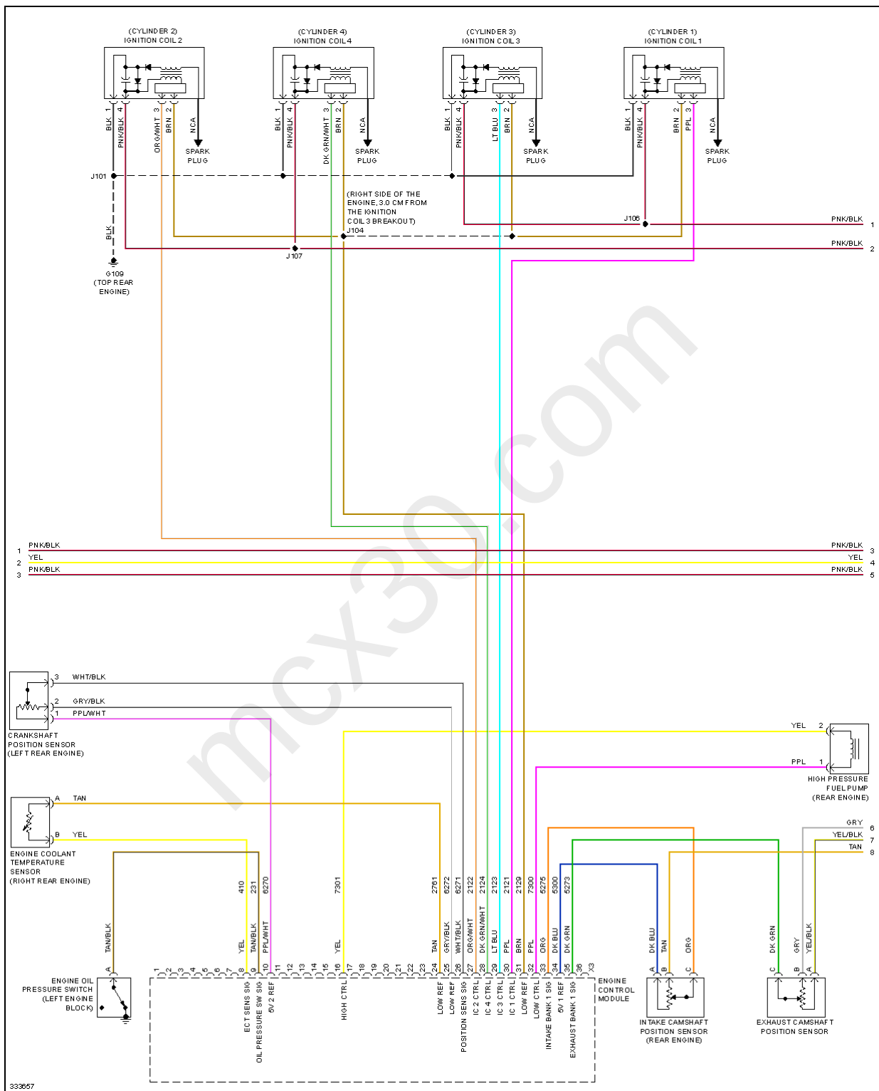
Fig. 21: 2.4L VIN W, Engine Performance Circuit (3 of 5)
