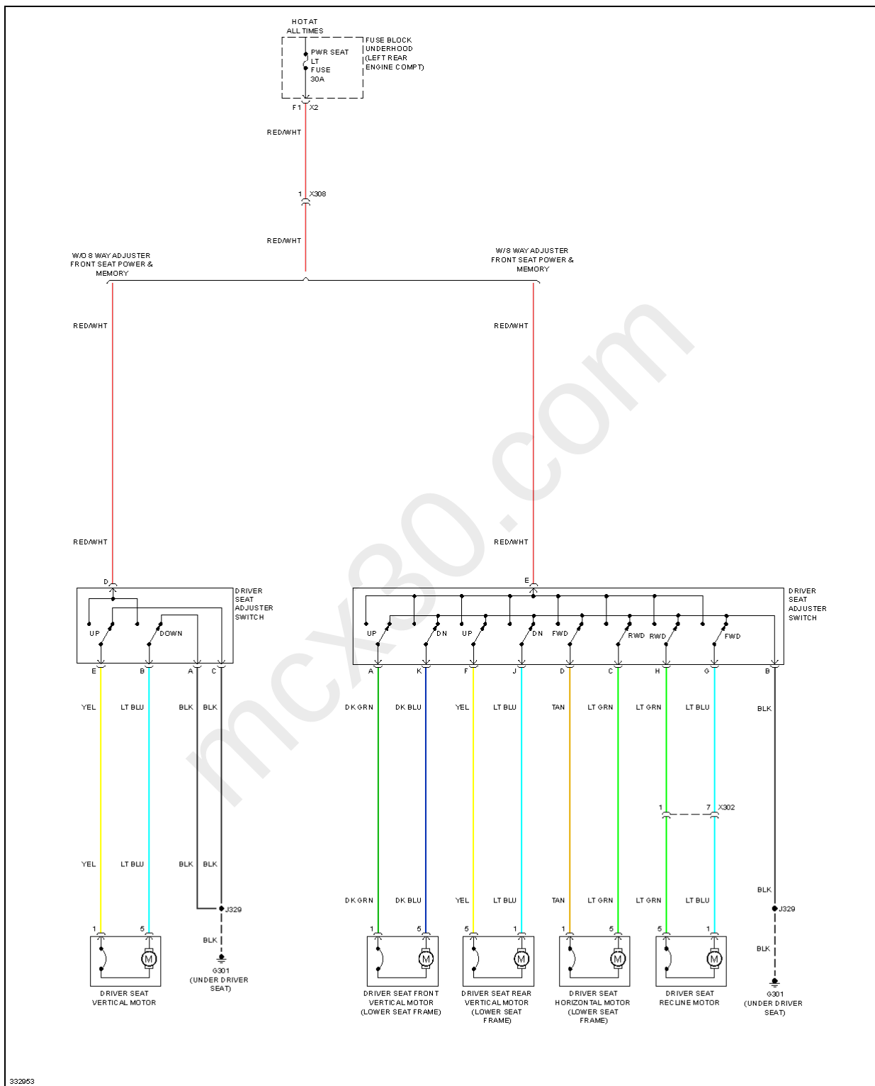
Fig. 62: Power Seat Circuit
