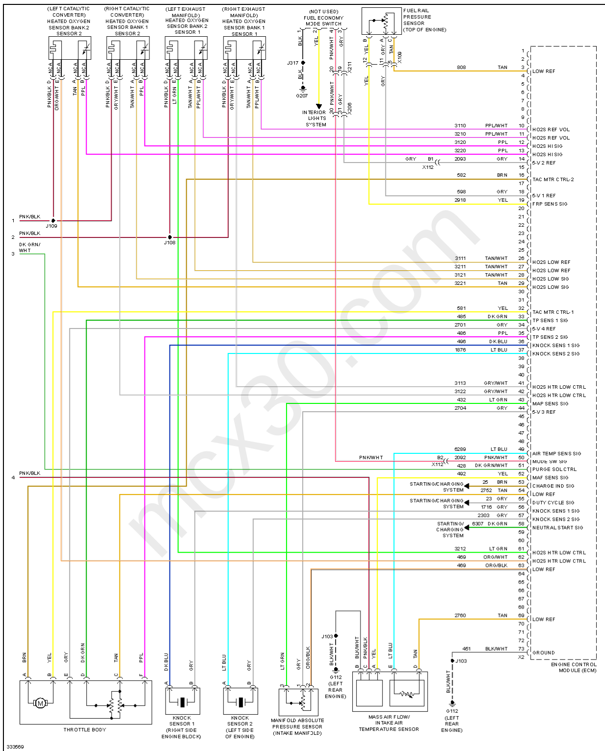
Fig. 28: 3.0L VIN Y, Engine Performance Circuit (5 of 5)
