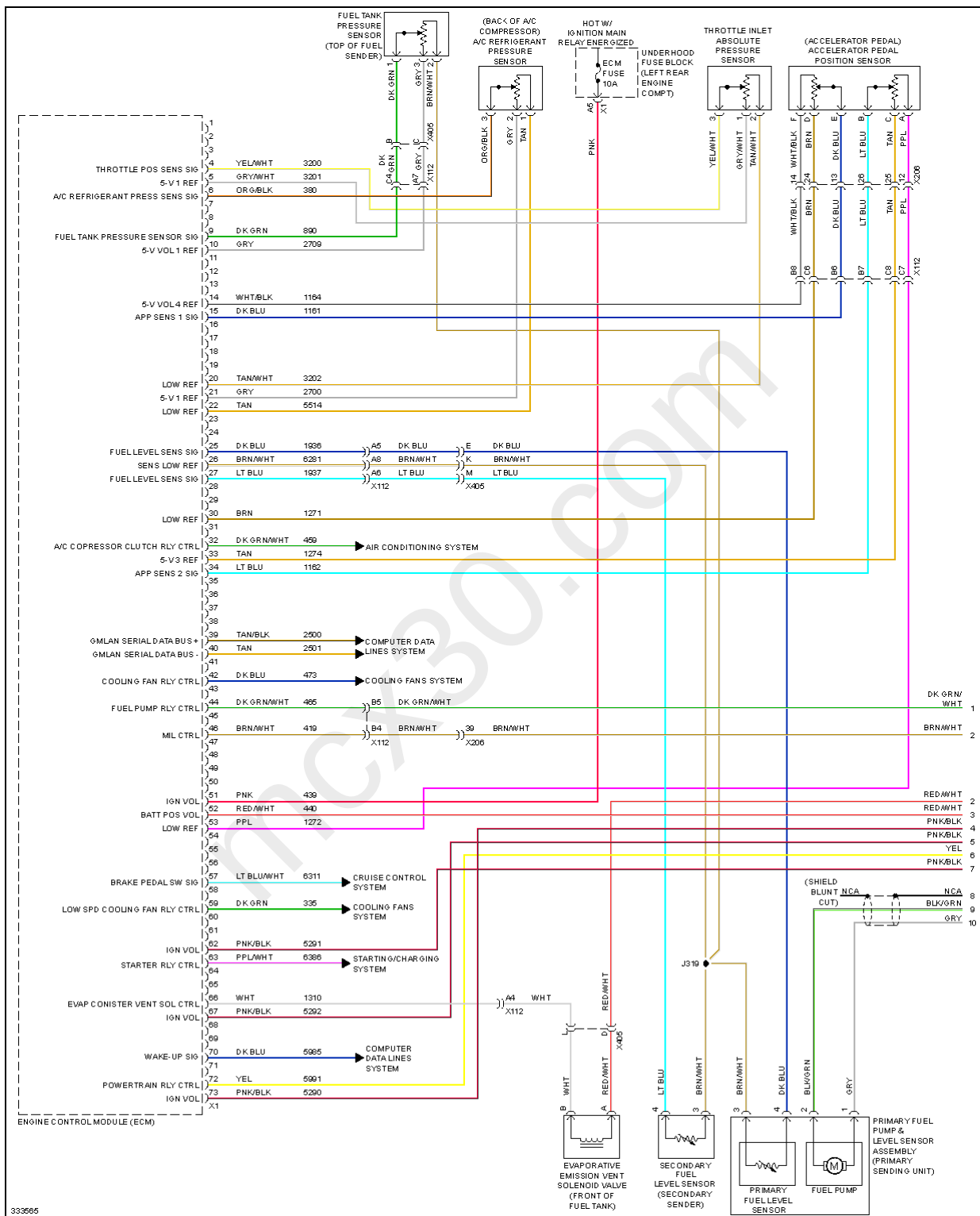
Fig. 24: 3.0L VIN Y, Engine Performance Circuit (1 of 5)
