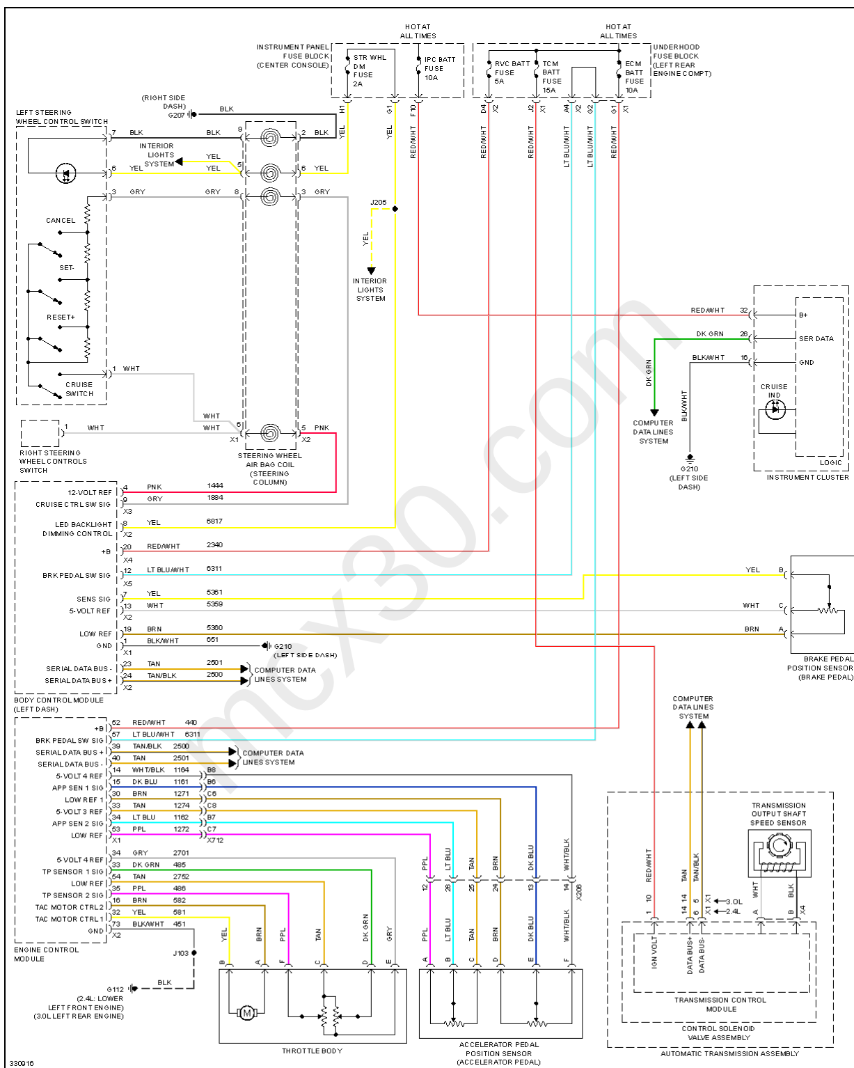
Fig. 16: Cruise Control Circuit
