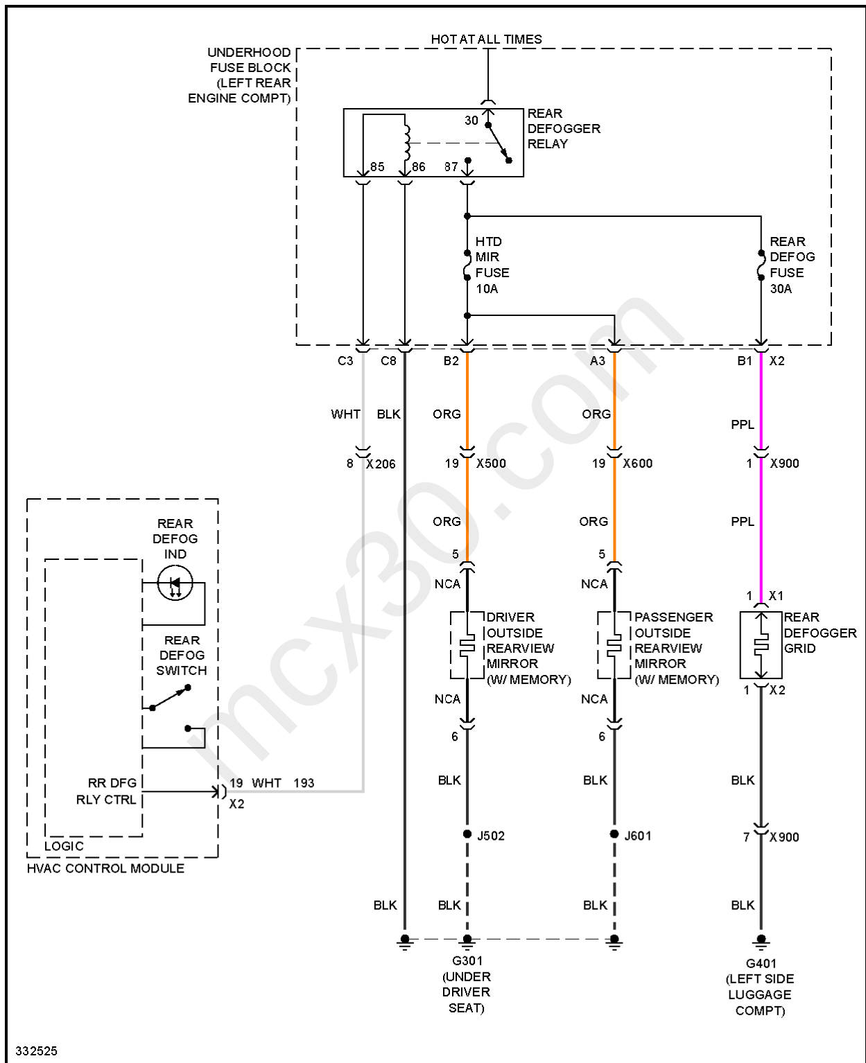
Fig. 17: Defoggers Circuit
