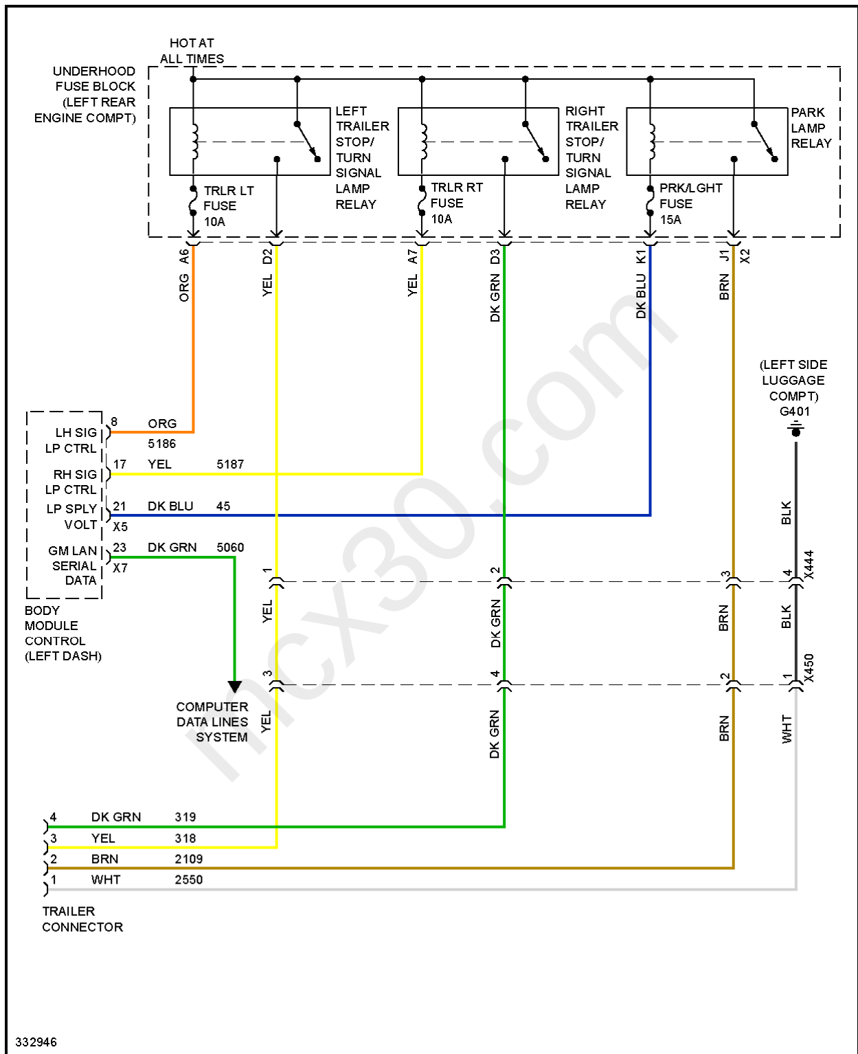
Fig. 31: Trailer Tow Circuit
