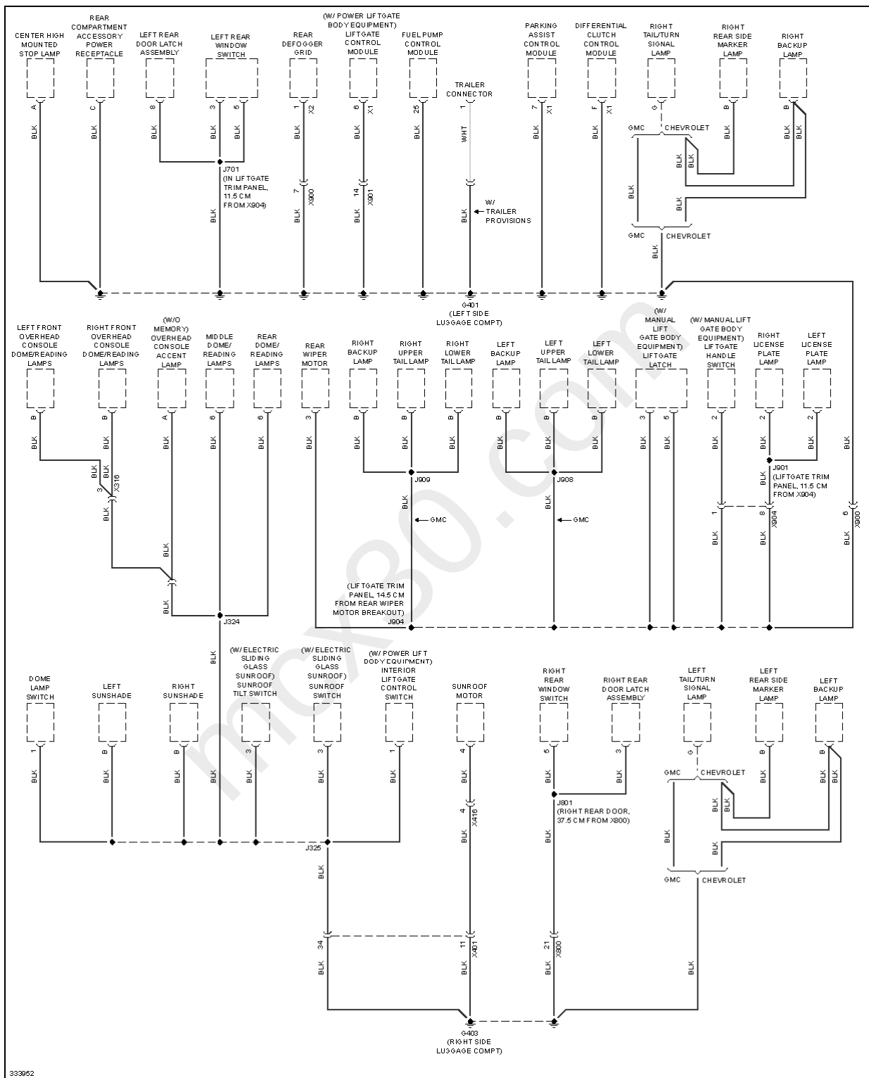
Fig. 35: Ground Distribution Circuit (4 of 4)
