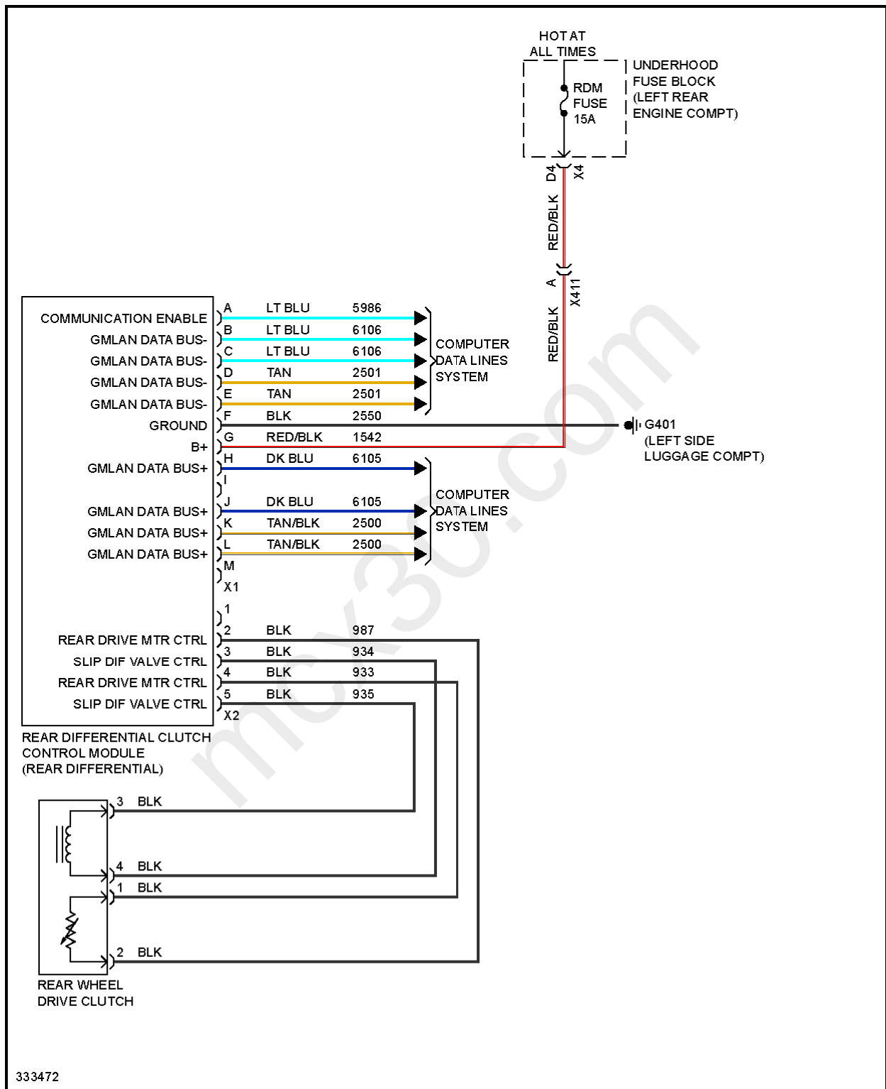
Fig. 78: 3.0L VIN Y, Rear Differential Lock Circuit
