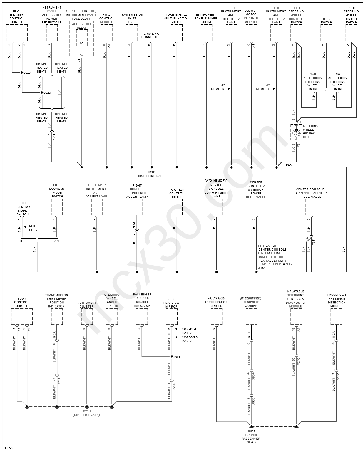
Fig. 33: Ground Distribution Circuit (2 of 4)
